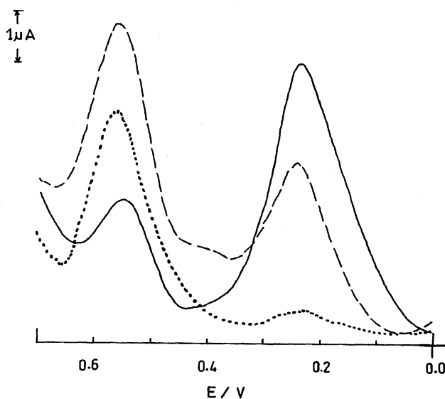
Fig. 3. Square wave voltammogram of P3MT/Fc film electrode in 0.1 M \text{H}_2\text{SO}_4 (supporting electrolyte). E_i=0.0 V, E_f=0.7 V, amplitude 25 mV, frequency=15 Hz, \Delta E=4 mV. 5.0 \times 10^{-5} M [\text{Fe}(\text{CN})_6]^{3-/4-} (—), 1.0 \times 10^{-4} M [\text{Fe}(\text{CN})_6]^{3-/4-} (---), 1.0 \times 10^{-3} M [\text{Fe}(\text{CN})_6]^{3-/4-} (....).
