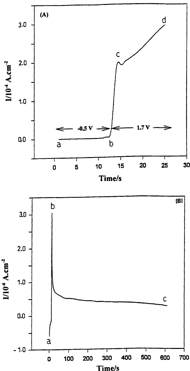
Fig. 1. (A) I - t transient curve for 0.05 \text{ M} 3MT, 0.05 \text{ M} FcPF in 0.10 \text{ M} TBAHP/AcN. E_i = -0.5 \text{ V} , E_f = +1.7 \text{ V} . (B) I - t transient curve for the polymer film formed under the same conditions as in Fig. 1A. Electrolyte is 0.10 \text{ M} TBAHP/AcN.
