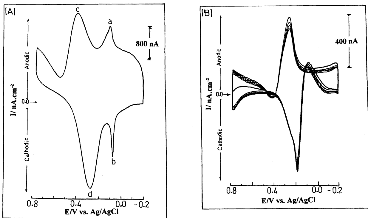
Fig. 2. (A) Cyclic voltammogram of P3MT/Fc film electrode in 1.0 mM [\text{Fe}(\text{CN})_6]^{3-/4-} in 0.1 M \text{H}_2\text{SO}_4 . Scan rate 50 \text{mV}\cdot\text{s}^{-1} . (B) P3MT/Fc electrode repeatedly cycled in 0.1 M \text{H}_2\text{SO}_4 for one hour. Scan rate 50 \text{mV}\cdot\text{s}^{-1} .
